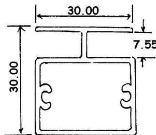
4175 0.530 KG/M
