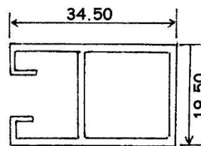
5591B 0.391 KG/M
