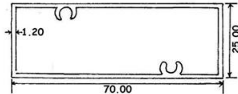
BX03272S 0.673 KG/M
