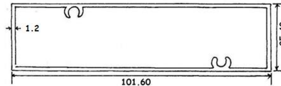
BX03132S 0.912 KG/M
