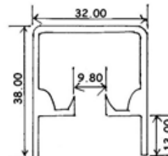
9203 0.555 KG/M
