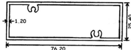
BX0310S 0.705 KG/M
