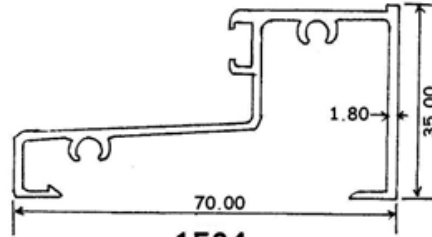
1584 0.825 KG/M
