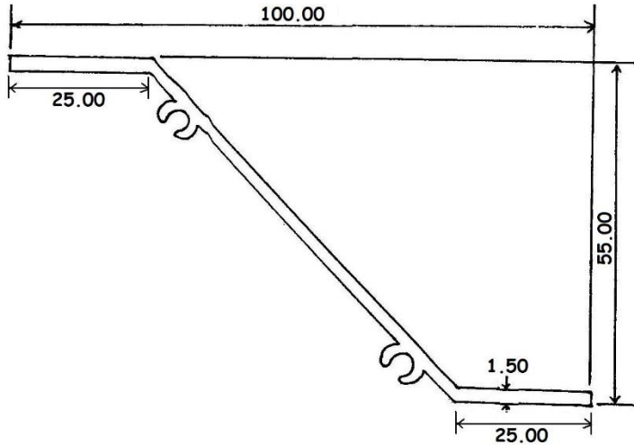
1558 0.580 KG/M
