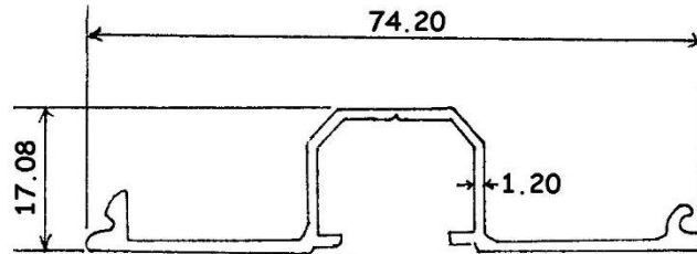
7502 0.416 KG/M
