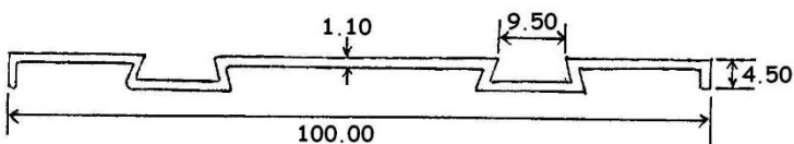
P5566 (SKIRTING) 0.400 KG/M
