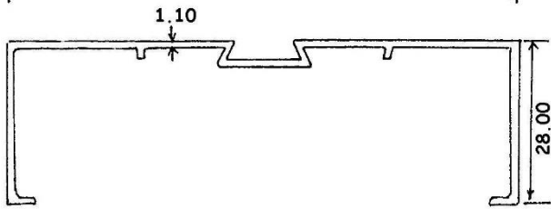
PGS20 (GLASS MOULD) 0.456 KG/M
